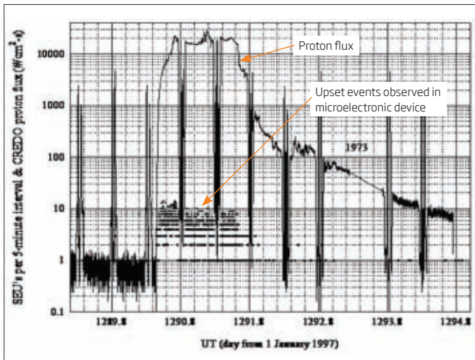
Figure 11: Observations of the onset of SEE on a satellite coincident with arrival of solar particles during Bastille Day event on 14 July 2000 – fluxes and SEE rates would be greater during an extreme event [Campbell et al., 2002]. Note that periodic dips and spikes in radiation are also observed since the observing satellite routinely crosses regions of radiation trapped by the Earth's magnetic field © QinetiQ
